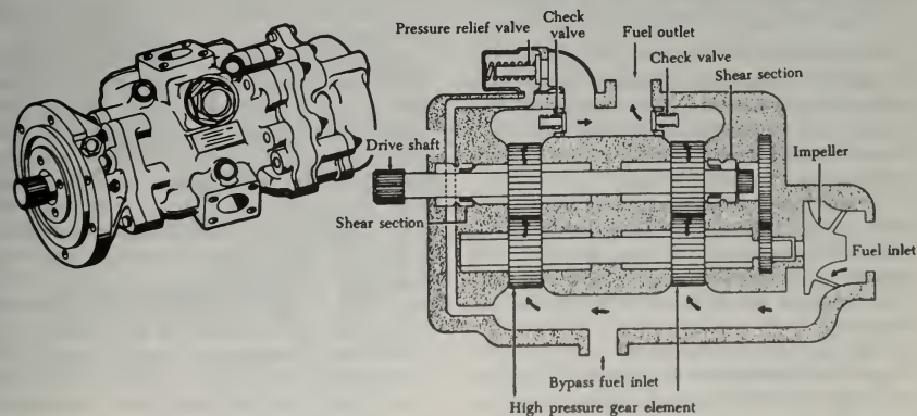
FIGURE 3-54. Engine-driven fuel pump.
